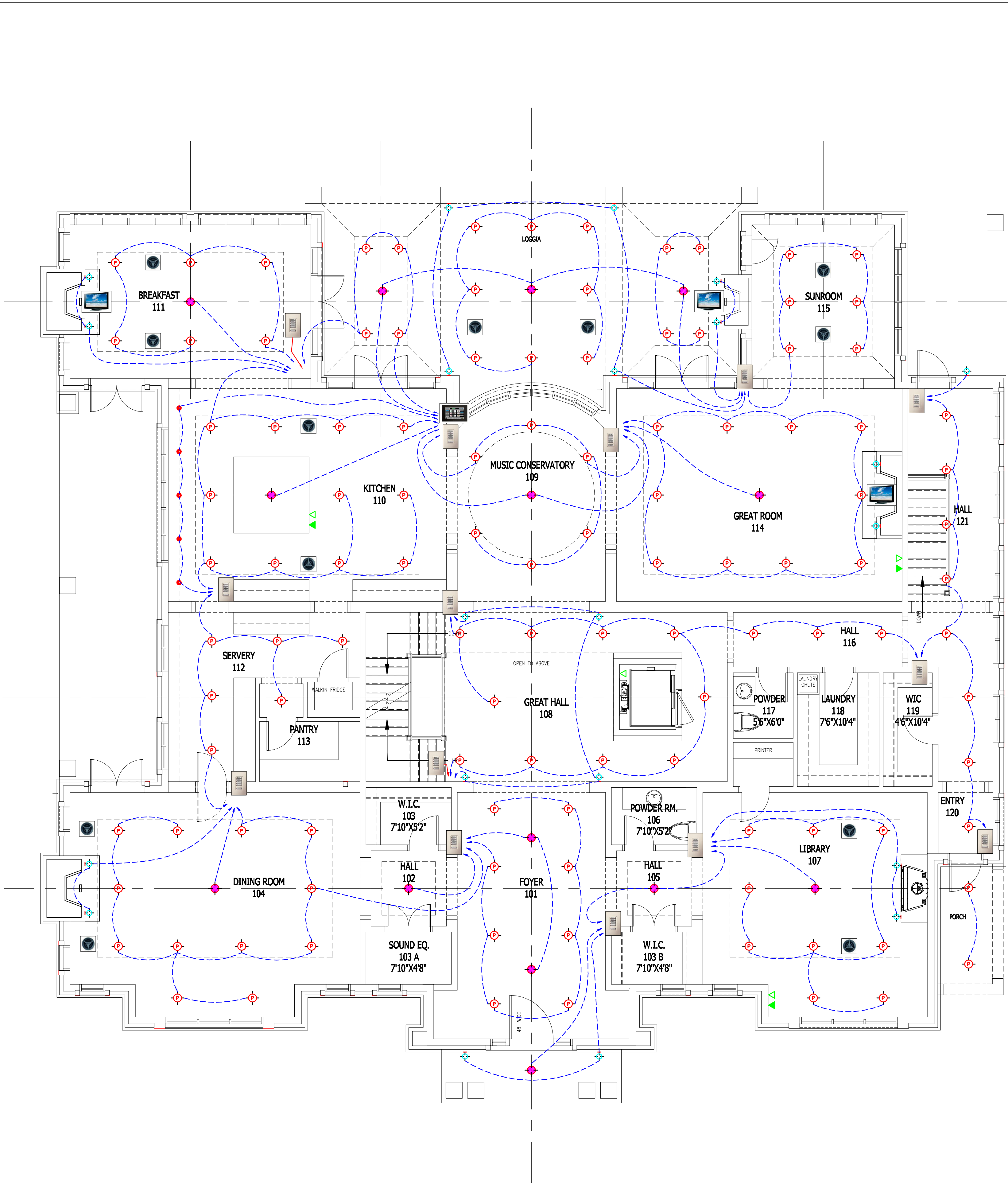
GROUND LIGHTING FLOOR PLAN SCALE: 1/4"=1'-0"
